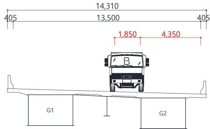
<Load Case 5>
