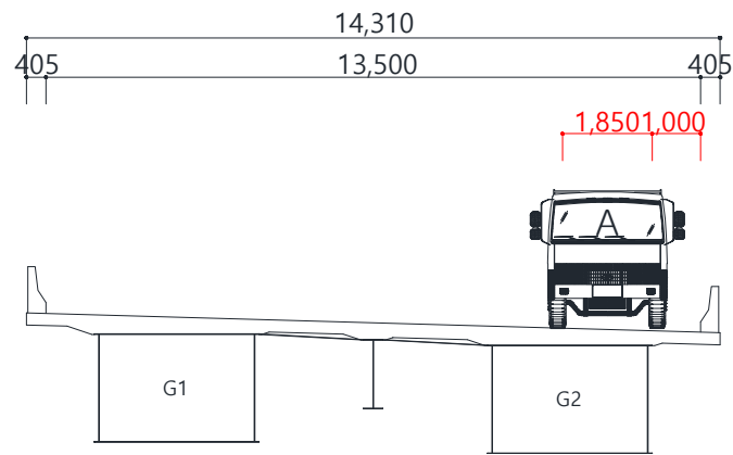
<Load Case 4>
