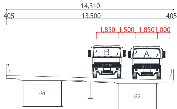
<Load Case 6>
